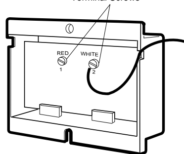
Multi-Function Door Control Panel Terminal Screws
