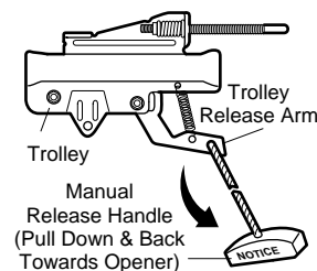
Lockout position
