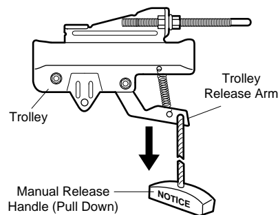
Lockout position
